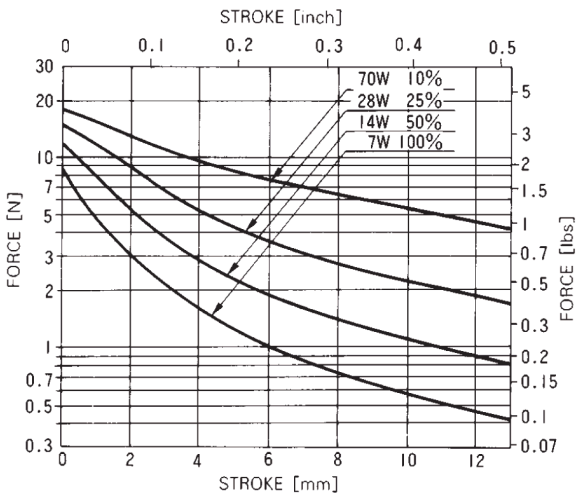
STROKE - FORCE
